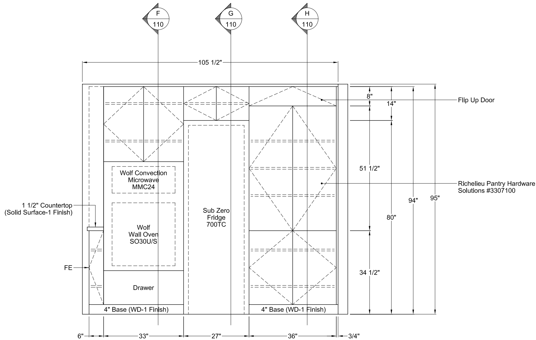
3 Kitchen Elevation 3 Scale As Shown
