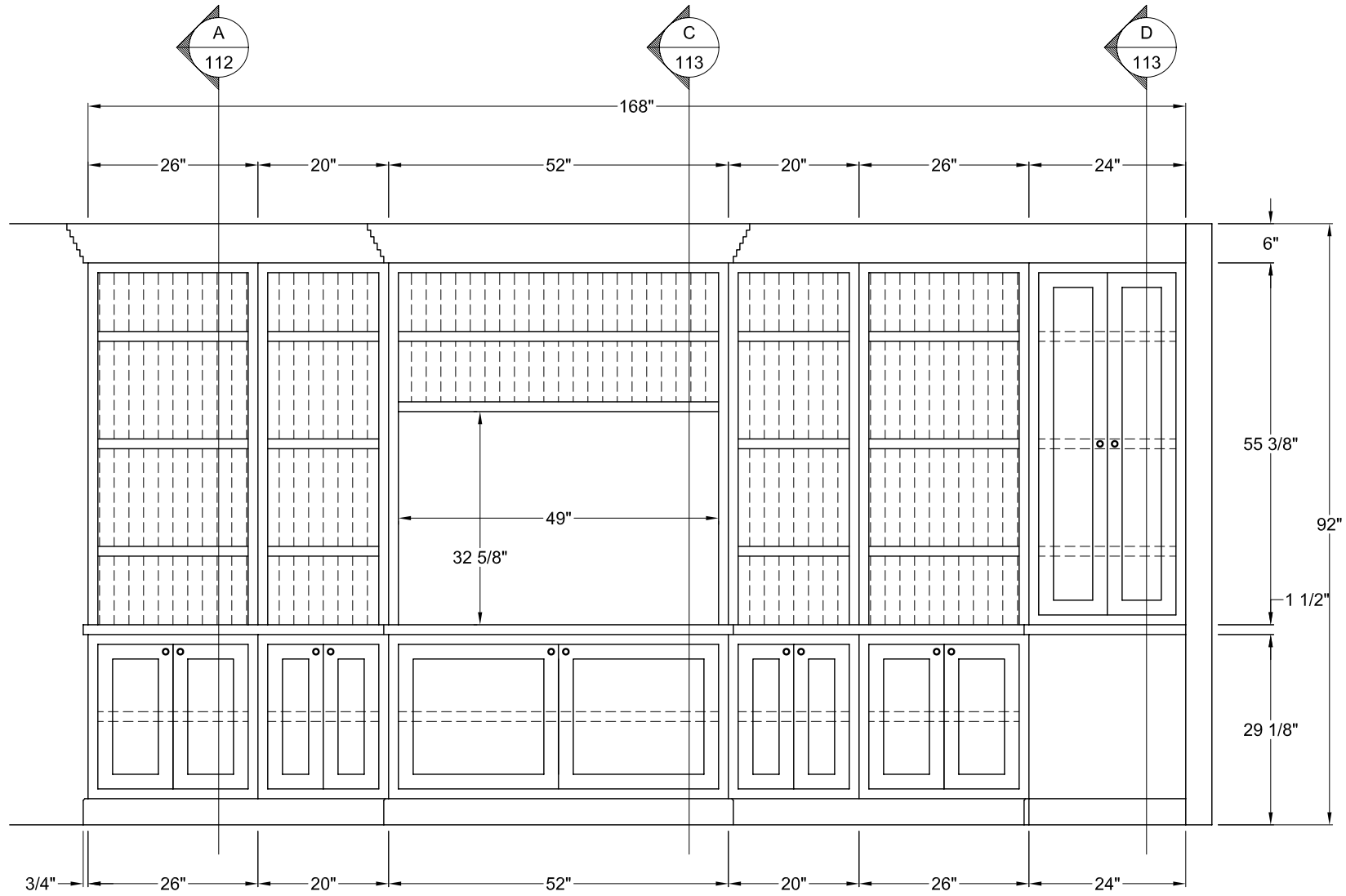
3 Upstairs Display and Desk Elevation 3 Scale As Shown
