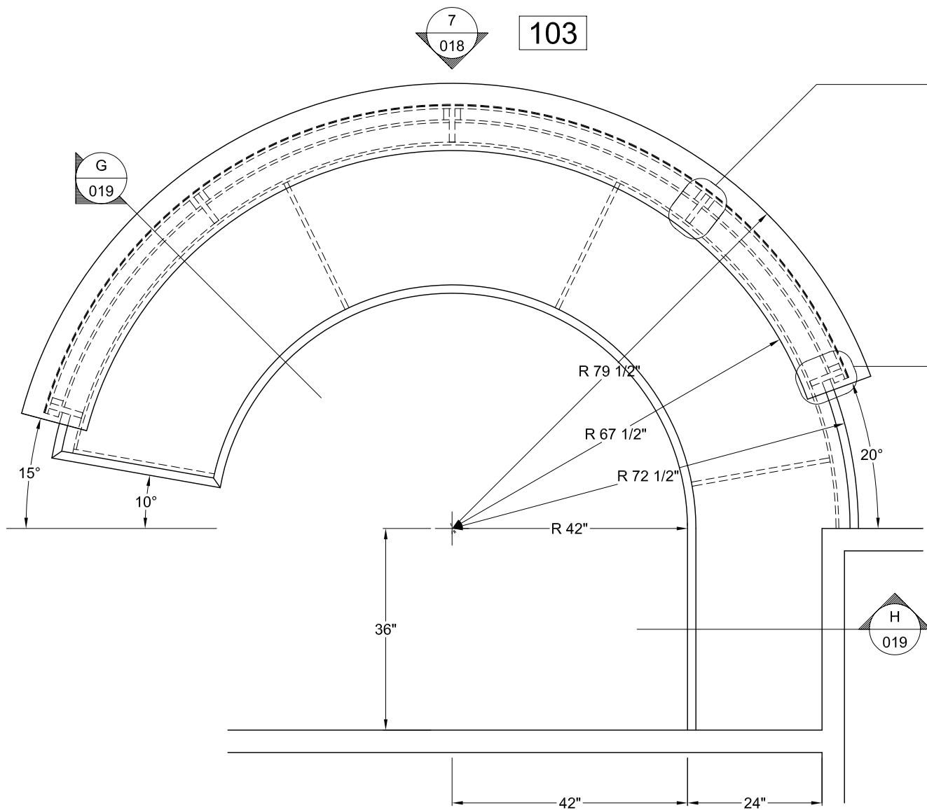
○ Rm 103 Reception Plan View Scale As Shown
