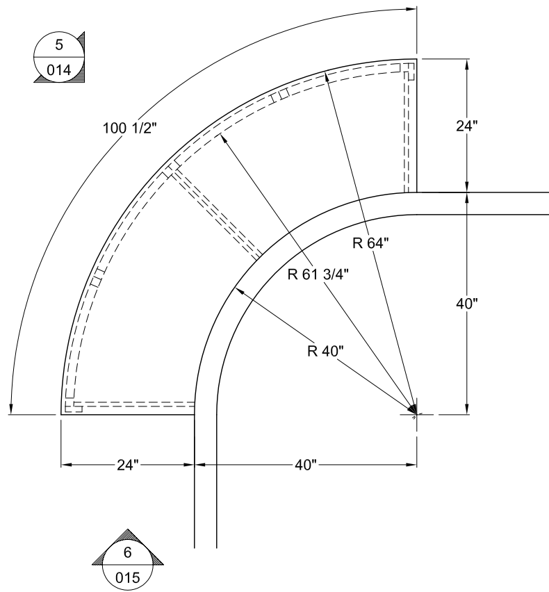
○ Rm 104 Coffee Counter Plan View Scale As Shown
