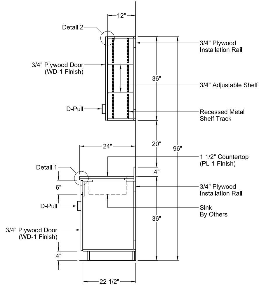
B Section B Scale As Shown
