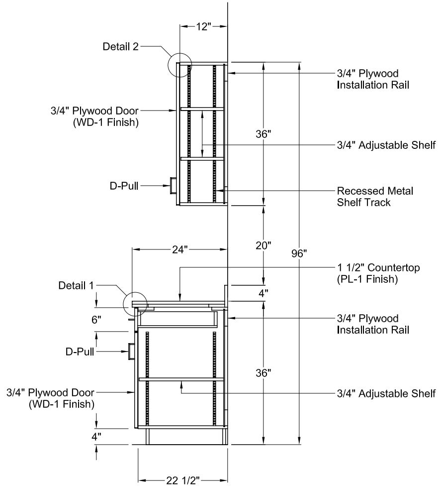
A Section A Scale As Shown
