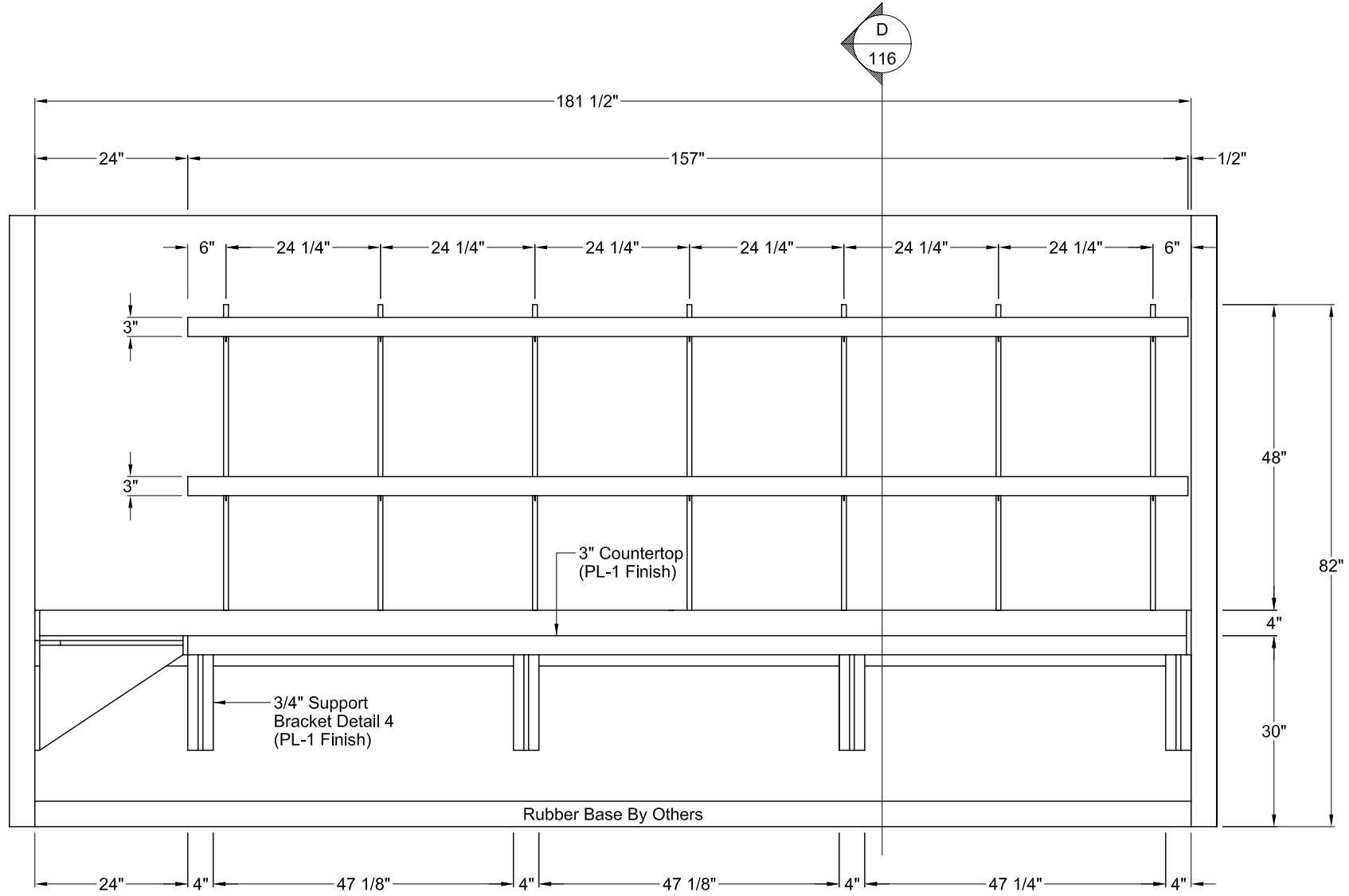
3 Rm 119 Storage / Charge Area Elevation 3 Scale As Shown
