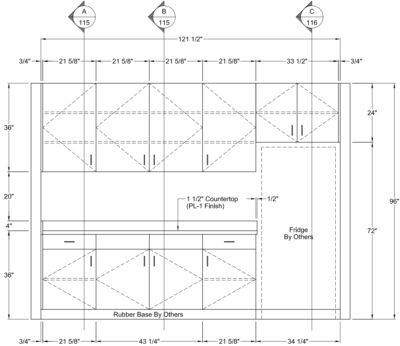
1 Rm 117 M.P.R. Elevation 1 Scale As Shown
