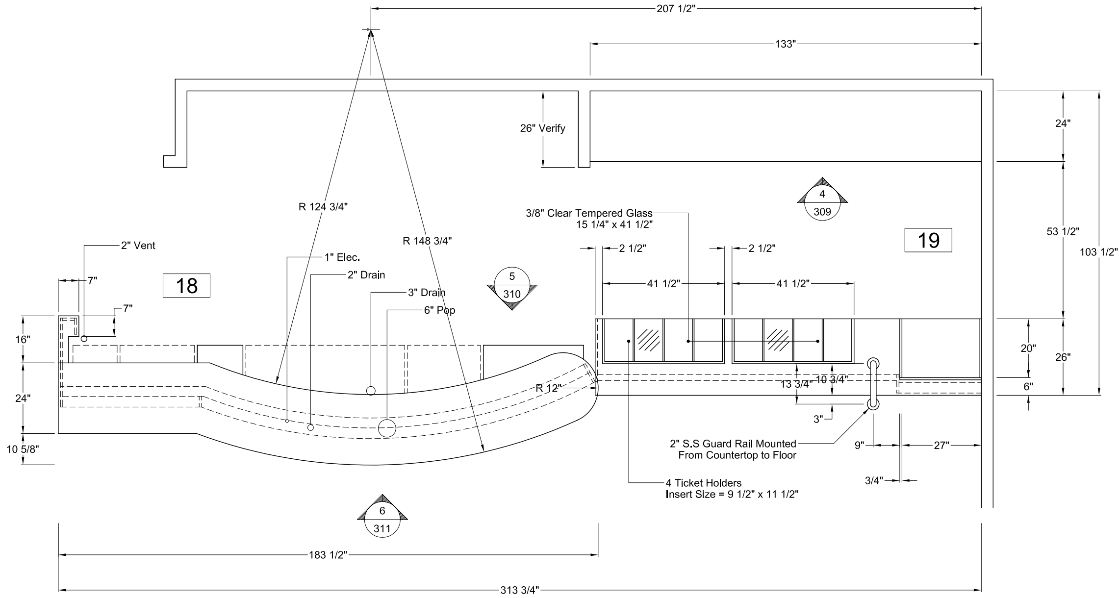
○ Rm 18 Bar and Rm 19 Gaming Centre Plan View Scale As Shown
