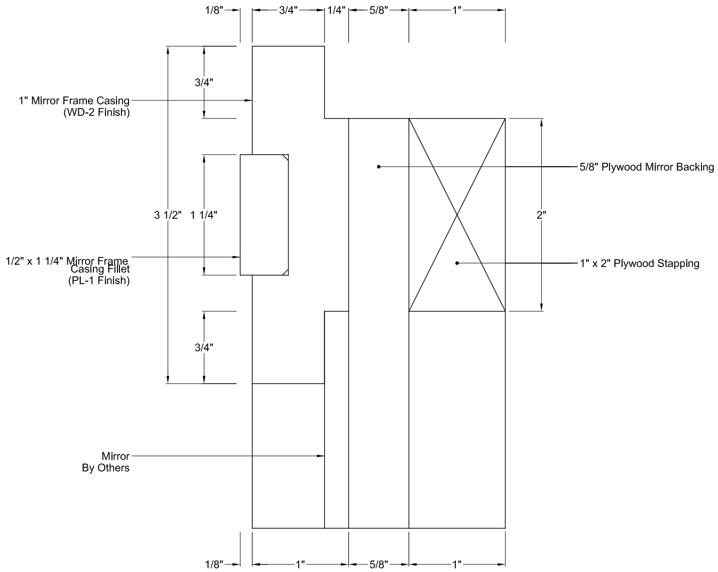
7 Detail 7 Scale As Shown
