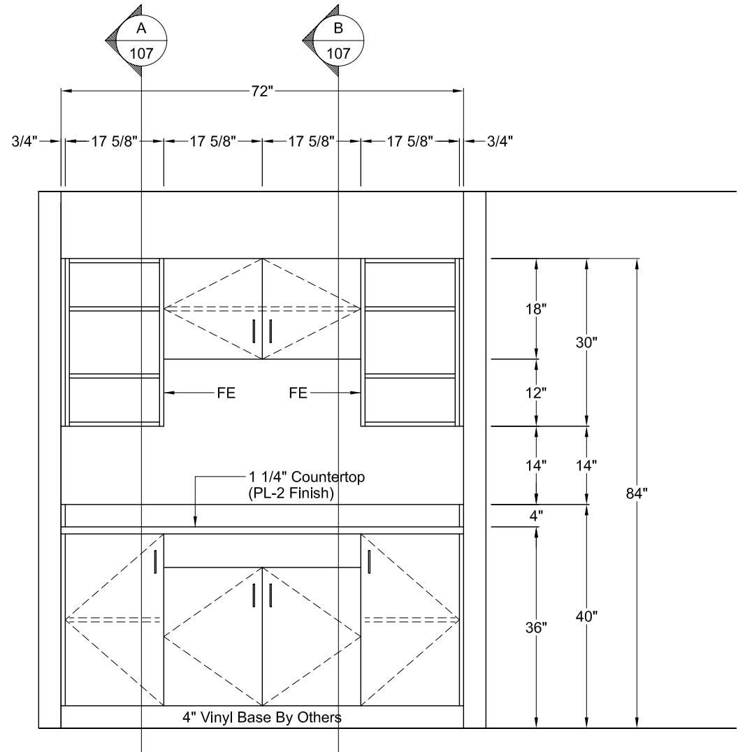
○ 1 Rm 04 First Aid Elevation 1 Scale As Shown
